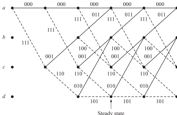
FIGURE 8.1-6 Trellis diagram for rate 1/3, K = 3 convolutional code.
