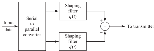
(a) Modulator
