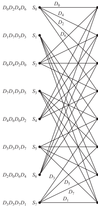
FIGURE 8.12-10 Eight-state trellis for rectangular QAM signal constellations.
