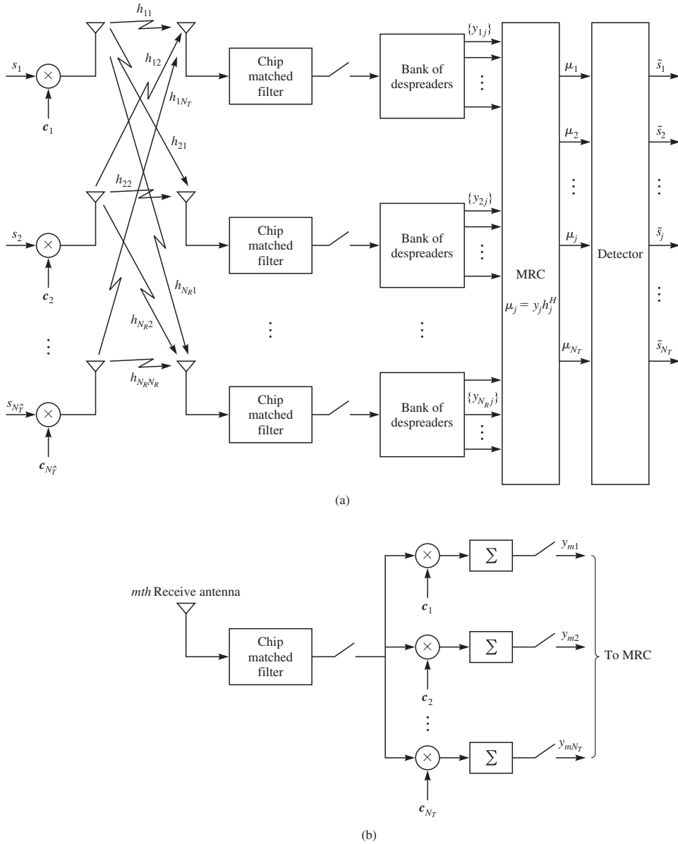
FIGURE 15.3-1 MIMO system with spread spectrum signals.
