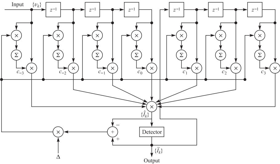
FIGURE 10.2-1 Decision-feedback equalizer.
