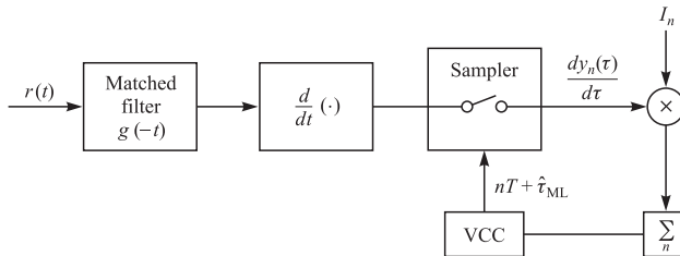
FIGURE 5.3–1 Decision-directed ML estimation of timing for baseband PAM.
