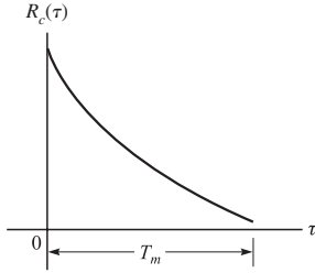
FIGURE 13.1-2 Multipath intensity profile.
