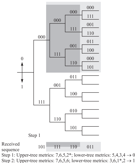
FIGURE 8.5-4 An example of feedback decoding for a rate 1/3 convolutional code.
