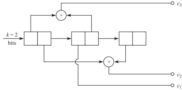
FIGURE 8.12-5 Rate \frac{2}{3} , eight-state trellis code.
