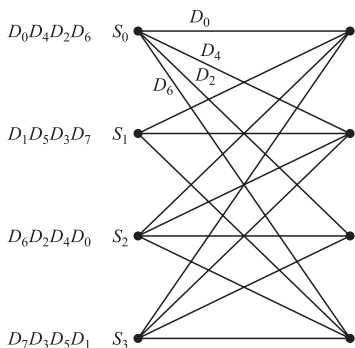
FIGURE 8.12–7 An alternative four-state trellis code.
