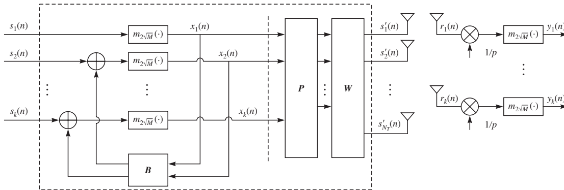
FIGURE 16.4-5 Tomlinson-Harashima precoding applied to a MIMO system.
