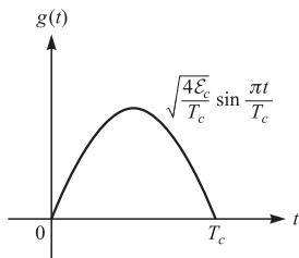
FIGURE 12.2-5 A sinusoidal signal pulse.
