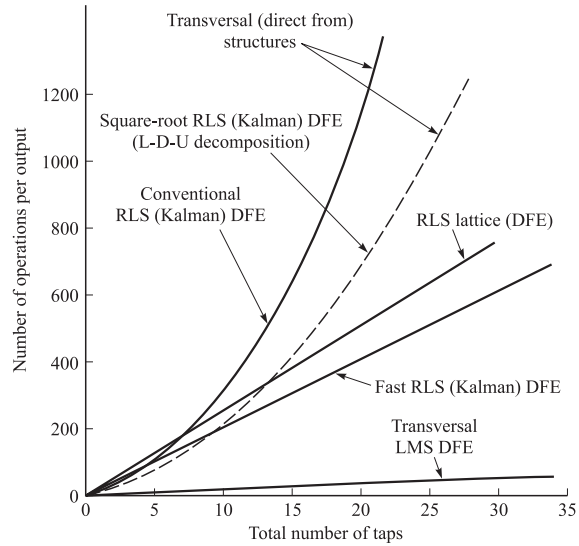
FIGURE 10.4-3 Computational complexity of DFE algorithms.
