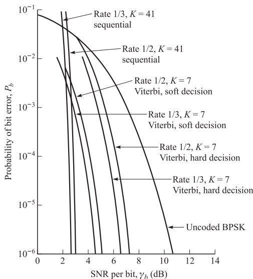
FIGURE 8.6-1 Performance of rate 1/2 and rate 1/3 Viterbi and sequential decoding. [From Omura and Levitt (1982) . © 1982 IEEE.]
