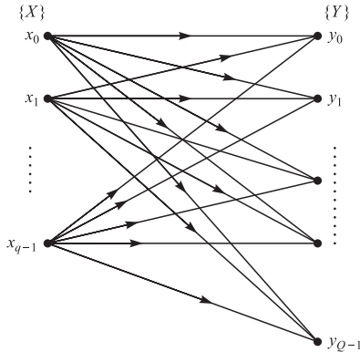
FIGURE 6.5-3 Discrete memoryless channel.
